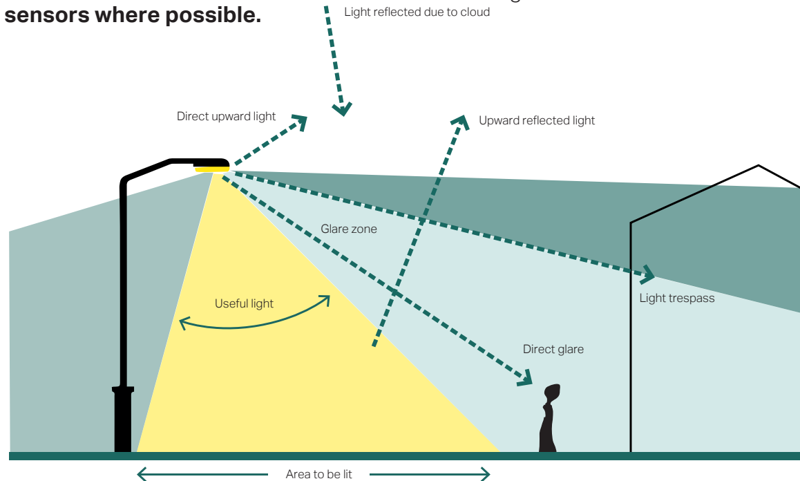
Figure 50: Diagram to illustrate the different components of light pollution and what 'good' lighting means
